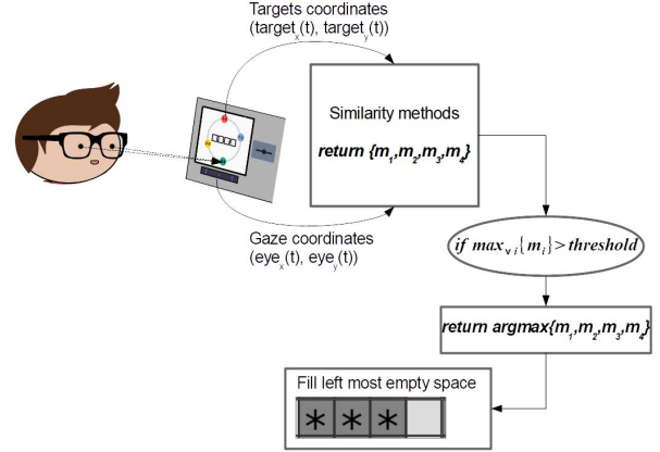
Fig. 4. PursuitPass architecture.
